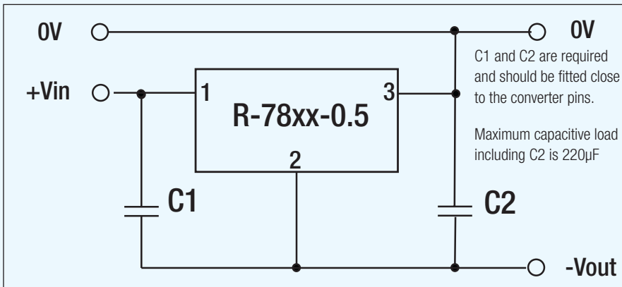
Pin Connections
